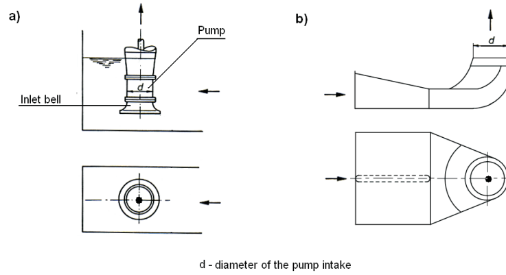
Figure 1 Suction intakes of pumps 1a) inlet bell 1b) formed suction intake
