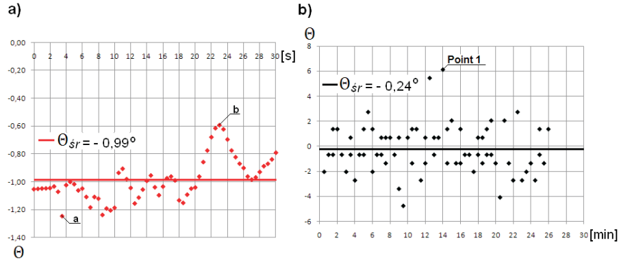
Figure 22 Change of the swirl angle in a function of time a) \theta(t) on the basis of measurement results b) set of points obtained on the basis of the number of rotations measurements of the swirl meter in a time of 30 minutes
