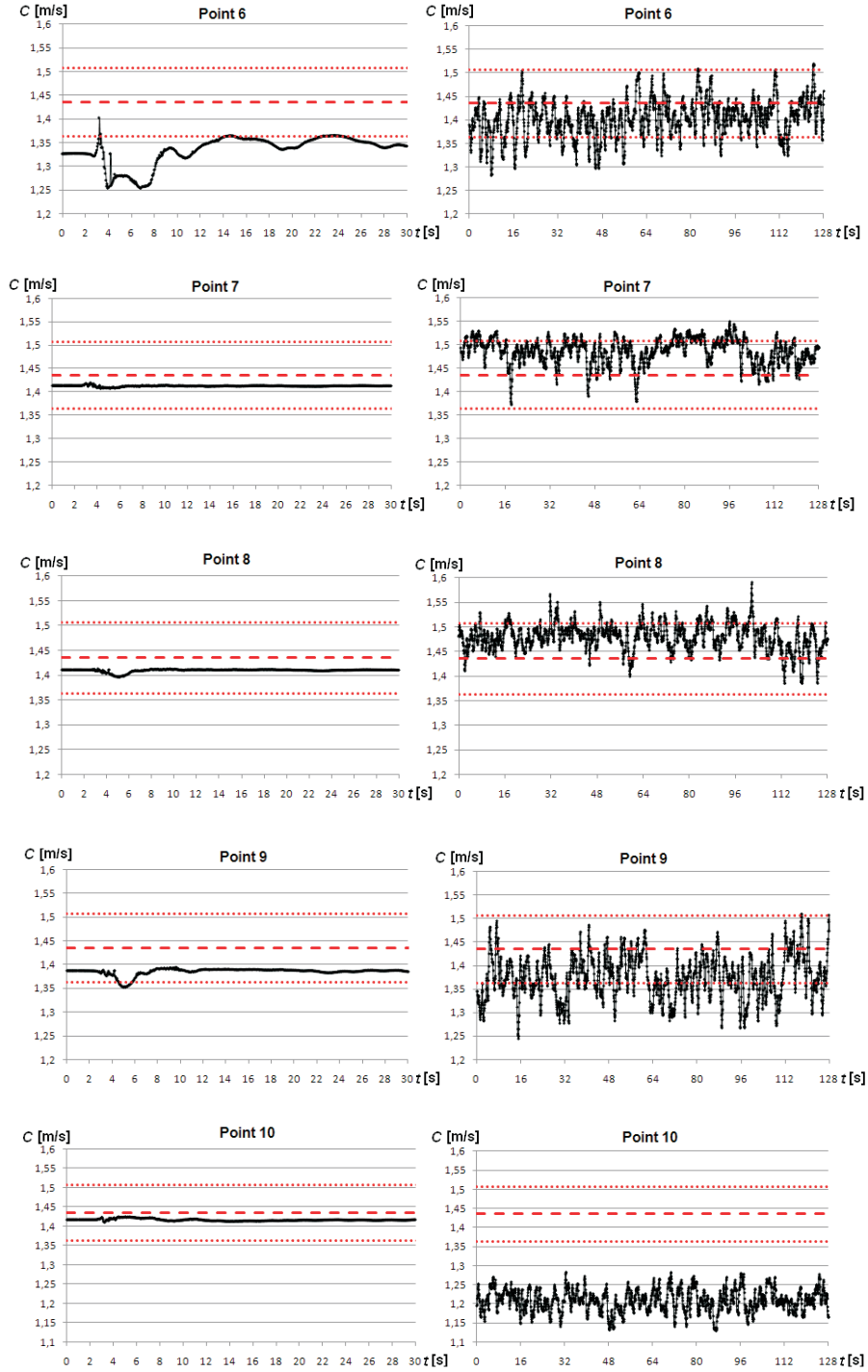
Figure 24 Changes of the velocity in points of the Pitot probe measurements in a function of time: a) according to numerical computations, b) from the Pitot probe measurements
