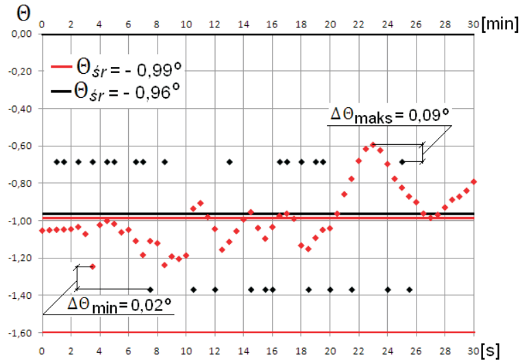
Figure 23 Course of the function of variety of the angle \theta in the period of 30 seconds on the basis of numerical computations. Black color points are the marked levels of minimum values of the angle \theta computed on the basis of measurements
