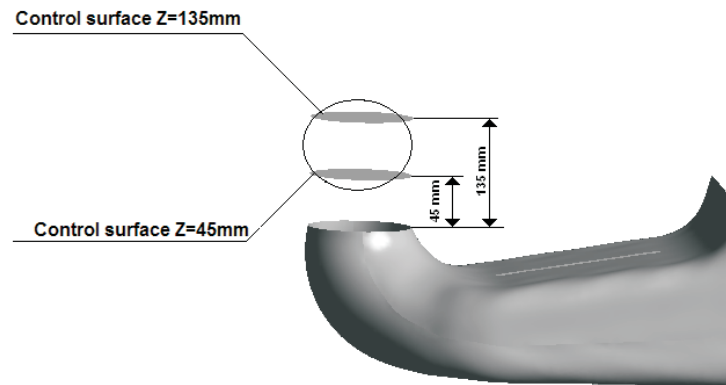
Figure 19 Measurement points of the Pitot probe in the outflow pipe
