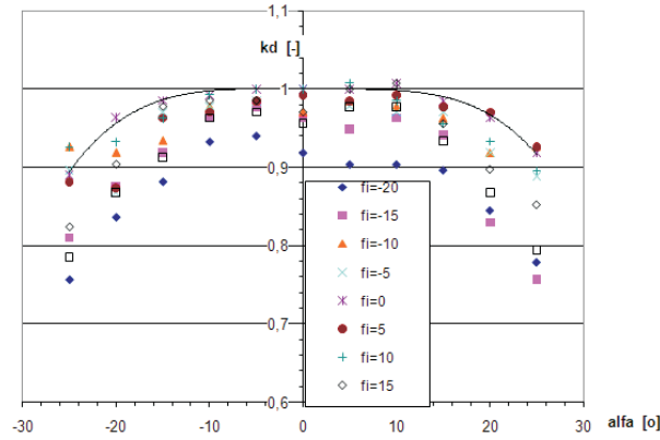
Figure 17 Directional characteristic of the Pitot probe
