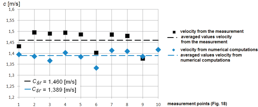
Figure 26 Averaged velocity values in points of measurements and computed numerically
