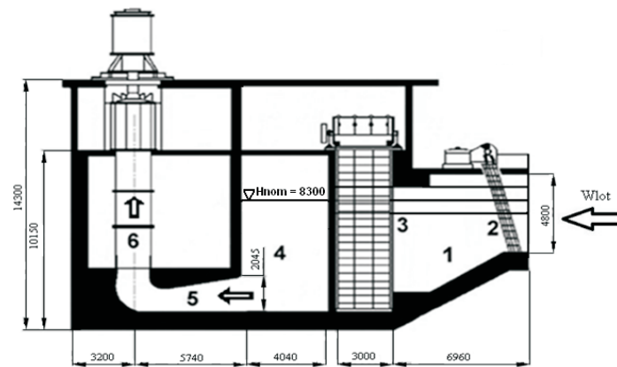
Figure 2 The real facility – system of intake channels [2, 3]
